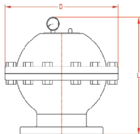
▲ Flang end (AIF) With Pressure Gauge
