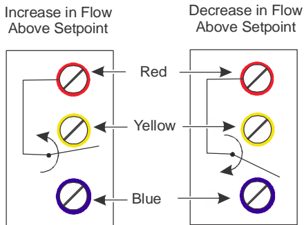
Figure 3: F261 Control Switch Action
